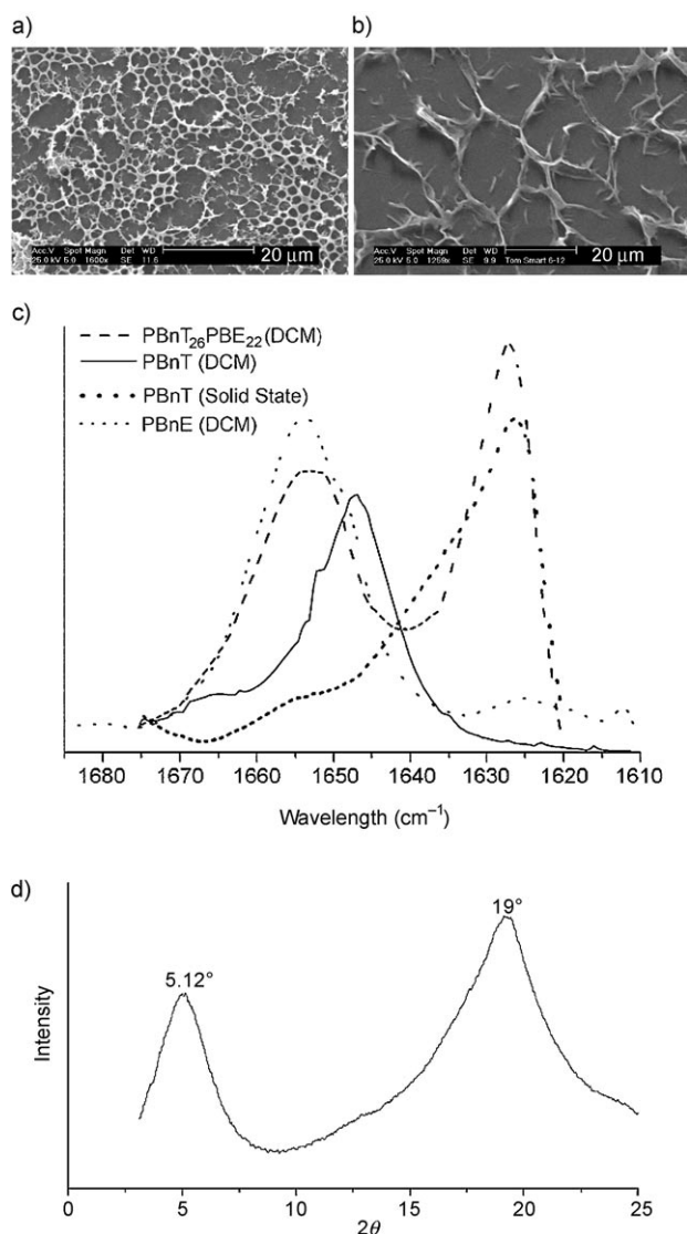
Figure 2. SEM images of dried-down samples of a) PBnT 16 -b-BnE 19 and b) PBnT 26 -b-BnE 22 . c) Infrared spectra of the amide I region of PBnT 26 -b-BnE 22 , PBnT, and PBnE in dichloromethane (DCM) and PBnT in the solid state. d) WAXS spectrum of PBnT 45 -b-BnE 18 .
